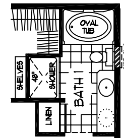
OPTIONAL BATH 1 (WITH 48" SHOWER, LINEN, AND EXTENDED LAVATORY)
