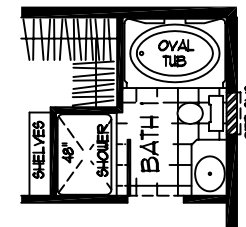
OPTIONAL BATH 1 (WITH 48" SHOWER)
