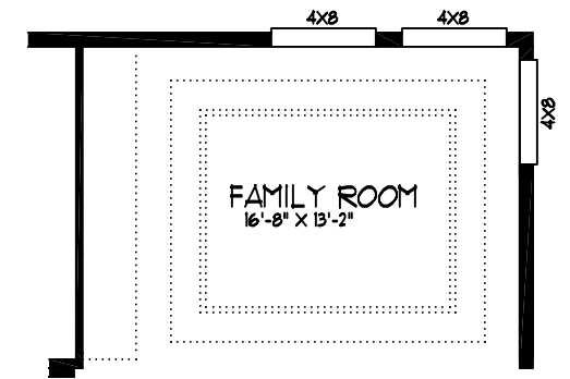
OPT. TOWER DORMER W/3 4x8 WINDOWS
